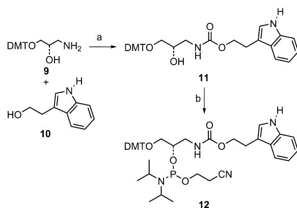
Scheme 3. Synthesis of In'-phosphoramidite 12 . Reagents and conditions: (a) CDI (1.1 equiv.), DMF, room temp., 3 d, 69%; (b) 2-cyanoethyl- N,N -diisopropylchlorophosphoramidite (1 equiv.), \text{EtN}(\text{iPr})_2 (3.6 equiv.), \text{CH}_2\text{Cl}_2 , room temp., 30 min, 96%.
