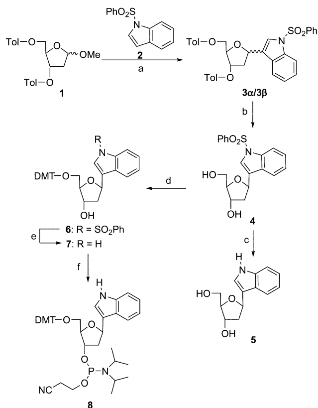
Scheme 2. Synthesis of In-phosphoramidite 8 . Reagents and conditions: (a) \text{BF}_3 \cdot \text{OEt}_2 (6.9 equiv.), \text{CH}_2\text{Cl}_2 , -15^\circ\text{C} , 1.5 h, 9% ( 3α ), 26% ( 3β ); (b) NaOMe (3 equiv.), MeOH, 6 h, room temp., 83%; (c) 18-crown-6 (1.5 equiv.), KOH (33 equiv.), MeOH, 1,4-dioxane, 2 h, room temp., 15%; (d) DMTCl (1.3 equiv.), \text{NEt}_3 (3 equiv.), pyridine, room temp., 16 h, 69%; (e) 18-crown-6 (1.5 equiv.), KOH (33 equiv.), MeOH, 1,4-dioxane, room temp., 16 h, 80%; (f) 2-cyanoethyl- N,N -diisopropylchlorophosphoramidite (1.5 equiv.), \text{NEt}_3 (3 equiv.), \text{CH}_2\text{Cl}_2 , room temp., 45 min, 95%.
