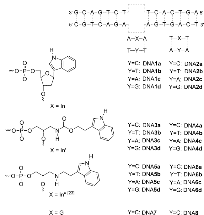
Scheme 4. Sequences of In-modified DNA1a–DNA2d, In'-modified DNA3a–DNA4d, In''-modified DNA5a–DNA6d [23] and unmodified duplexes DNA7 [23] and DNA8. [23]
