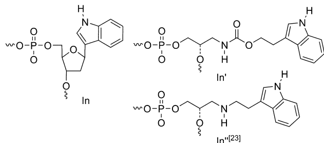
Scheme 1. Structural variations to incorporate indole as an artificial base into oligonucleotides.
